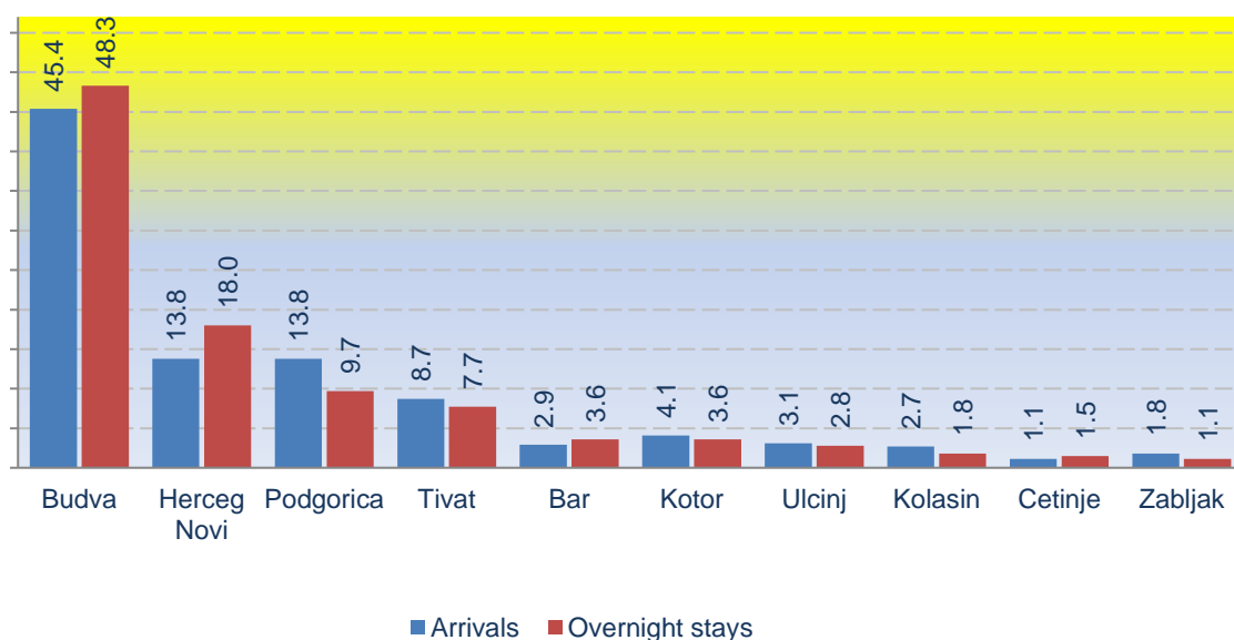
Graph 2 Structure of arrivals and overnight stays of tourists in collective accommodation in the most visited municipalities (in %), April 2019
