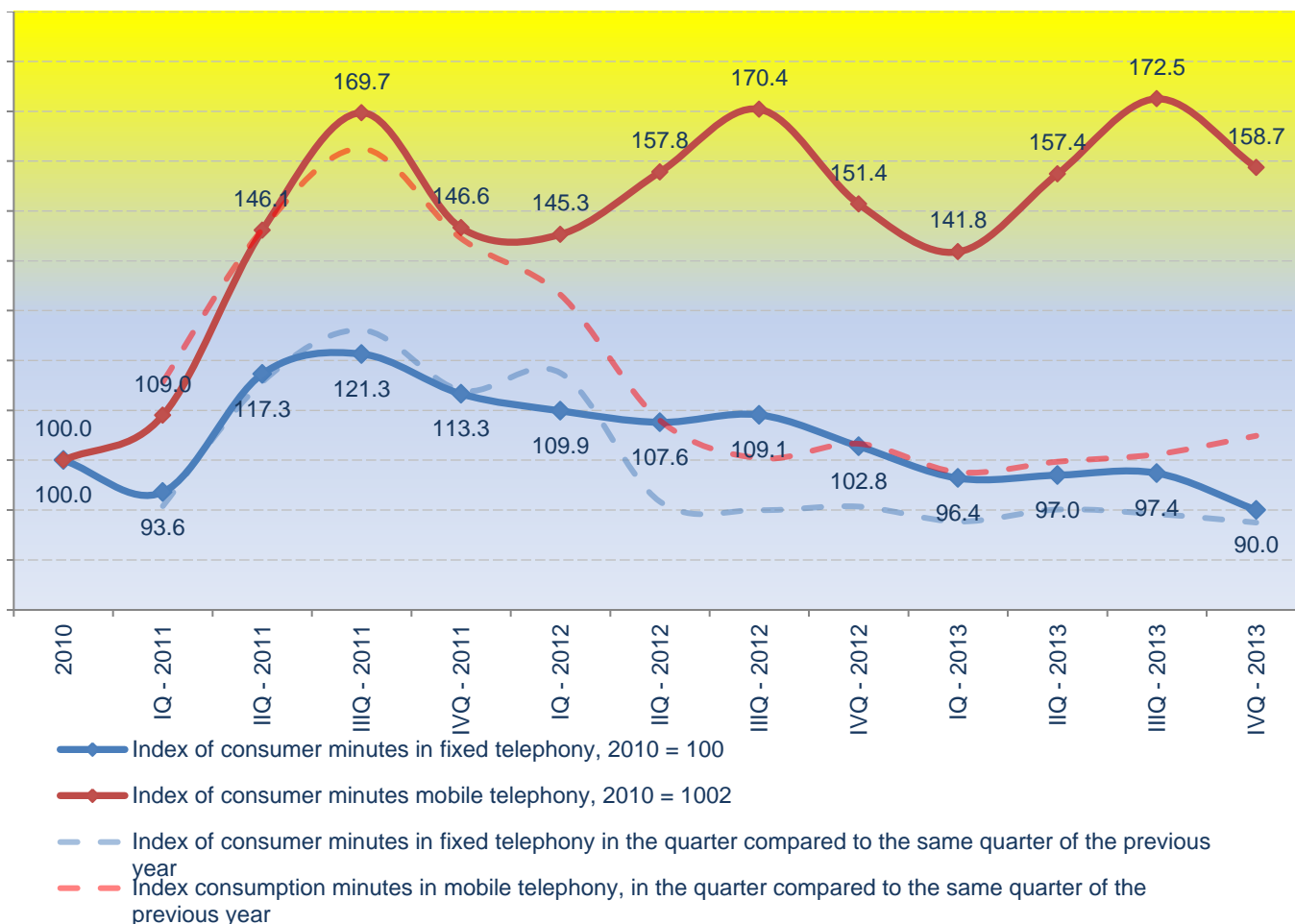
Graph 1. Indices of fixed and mobile telecommunication minutes
