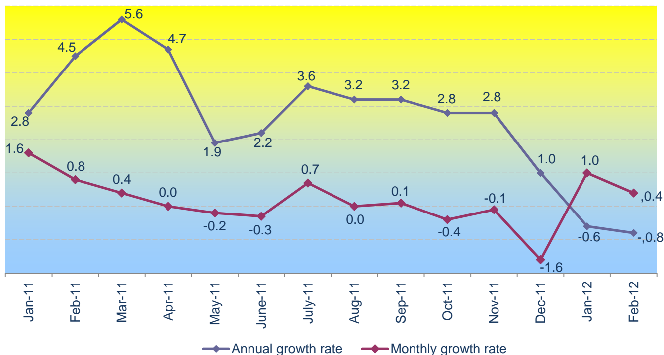
Growth rate of producer prices, in %
